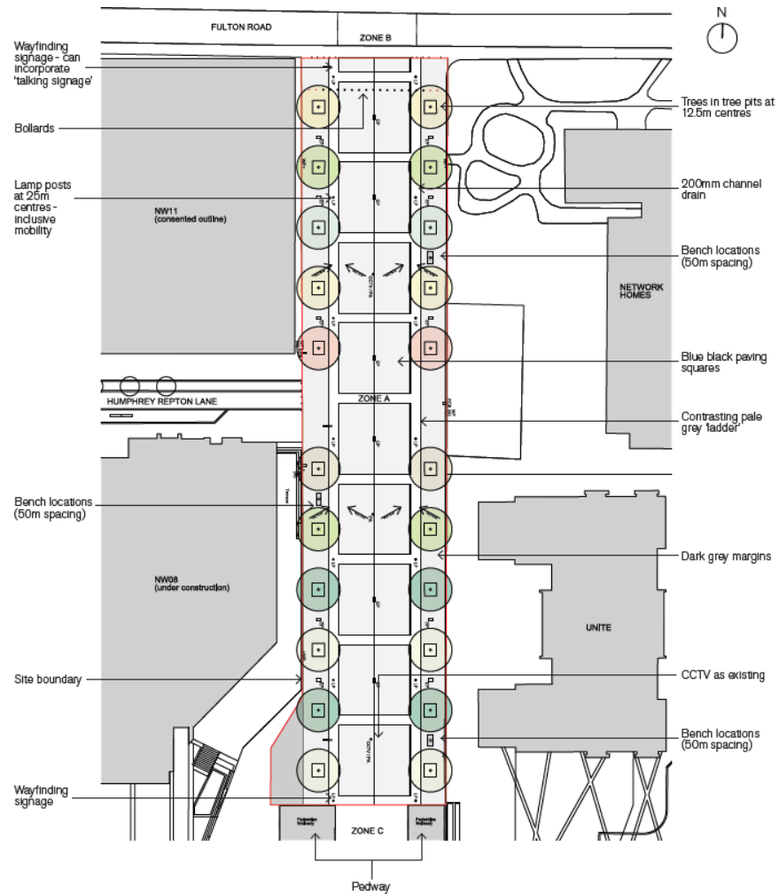
Proposed plan of Zone A showing site boundary, trees, paving pattern, drainage and paving falls.
